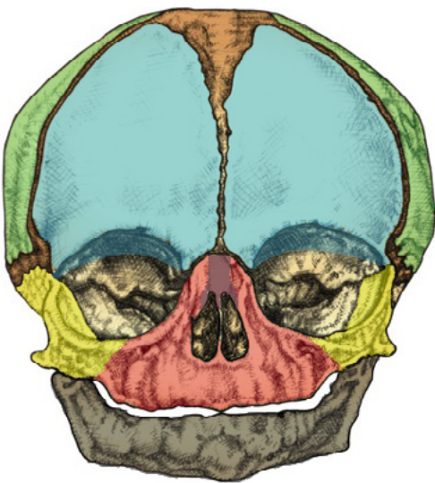
PLAN FRONTAL
