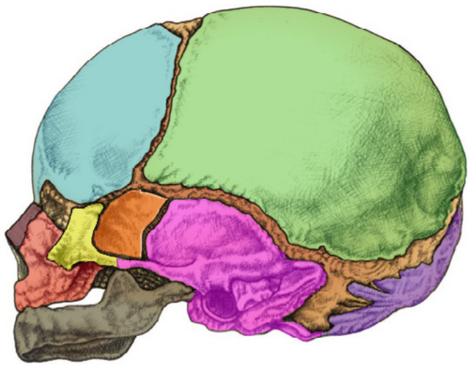
PLAN SAGITTAL
