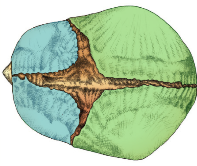
PLAN AXIAL
