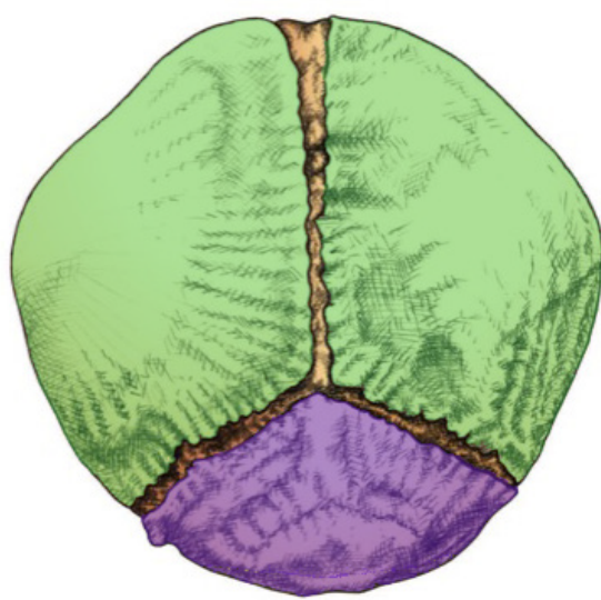
PLAN OCCIPITAL
